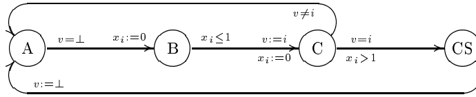
Fig. 3. Fischer's protocol for mutual exclusion
