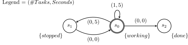
Figure 2: n -WKS illustrating working on a set of tasks
