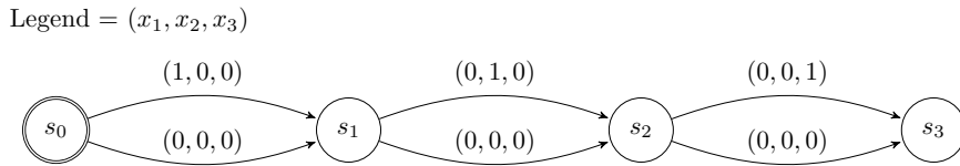
Figure 4: Encoding of variable assignment
