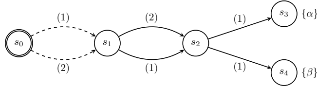
Figure 7: Illustrating memory requirements
