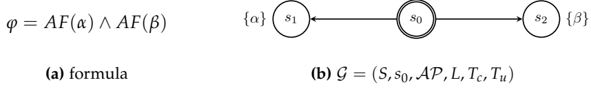
Figure 10: n -WG (\mathcal{G}, \varphi) illustrating a game with separate winning strategies for each subformula
