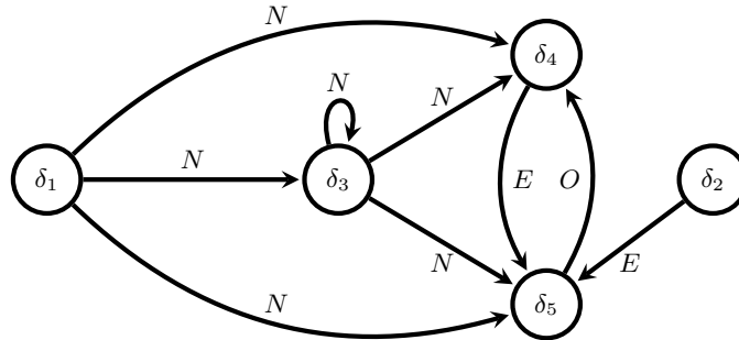
Fig. 2. The directed graph formed by the rules to compute naturals, evens, and odds
