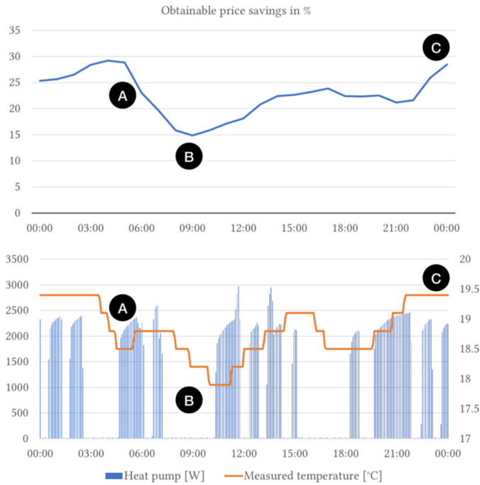
Fig. 5. Data collected from Household E over 24 hours on 18 April 2016. The top graph shows the obtainable price savings. The bottom graph shows the measured indoor temperature (orange line), and the electricity consumed by the heat pump (vertical blue bars).
