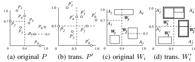
Fig. 1. HSD Transformation Example, E = 2
