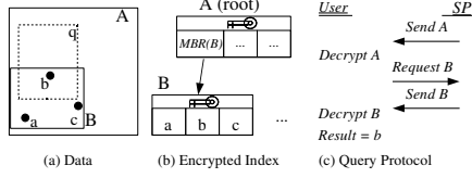
Fig. 2. Query Processing in CRT
