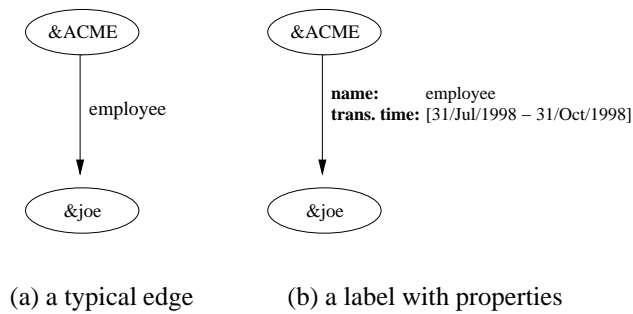
Figure 1: The New Kind of Edge Labels
