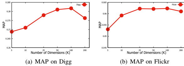
Fig. 7. Effect of number of dimension K on Digg and Flickr.
