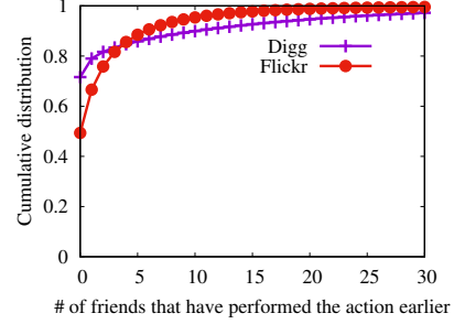
Fig. 3. The CDF of taking an action after x friends have performed the action.
