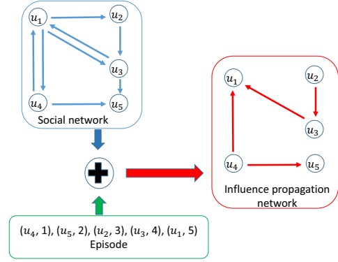
Fig. 5. An example of building influence propagation networks.
