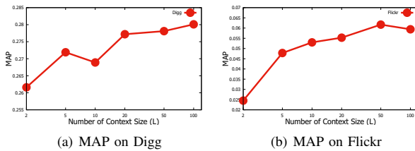
Fig. 8. Effect of context size L on Digg and Flickr.
